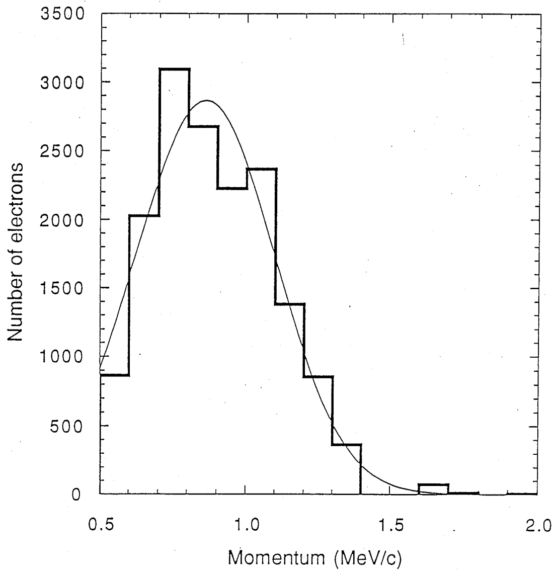
Fig. 2. Momentum spectrum of electrons produced by the 200 ps laser pulse at the injection bending field set to 1 MeV/c. The solid line shows a fit to a Gaussian distribution.
