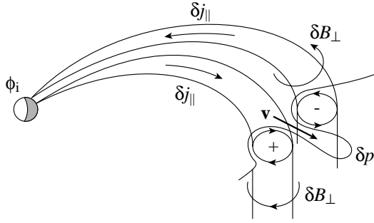
Figure 1. Geometry of the unstable growth of the localized pressure fluctuation \delta p due to the interchange instability. The magnetic field is dragged with the convection due to the frozen in condition, which in turn generates the symmetry breaking of the region 1 currents to form the substorm current wedge.
