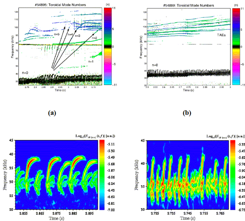
Figure 1. Frequencies for various toroidal n -numbers picked up by magnetic Mirnov signals in JET discharges: (a) #54895 and (b) #54899. Zooms of the frequency of the n = 0 mode are shown in (c) and (d) for discharges #54895 and #54899, respectively. In the legends of (c) and (d) S_{\delta B}(t, f) is the short-time Fourier transform of \delta B with arbitrary units for \delta B and S .
