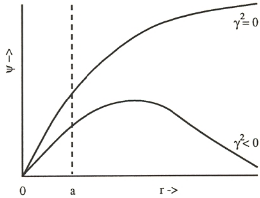
Figure 2: A schematic diagram showing how the large r boundary condition is satisfied when the marginally stable test solution does not cross the axis.
