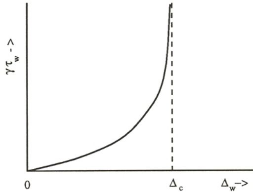
Figure 6: A schematic diagram showing the typical variation of the growth rate with the shell stability index for a partial shell.
