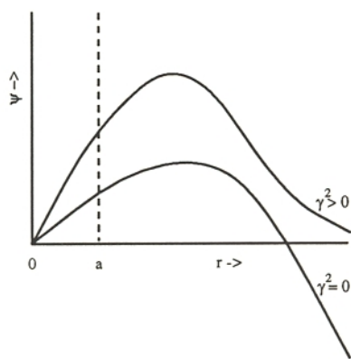
Figure 3: A schematic diagram showing how the large r boundary condition is satisfied when the marginally stable test solution crosses the axis.
