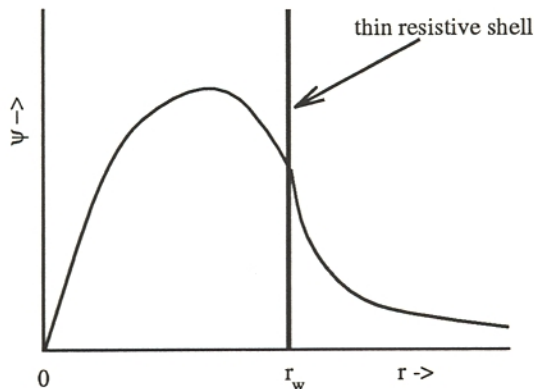
Figure 4: A schematic diagram showing a typical resistive shell mode solution.
