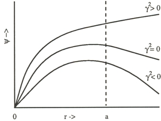
Figure 1: A schematic diagram showing the relationship between unstable, oscillatory, and marginally stable test solutions.
