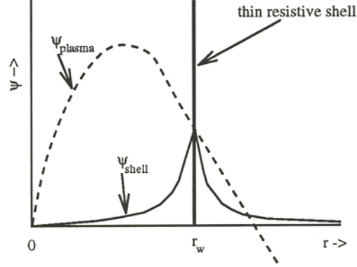
Figure 5: A schematic diagram showing the plasma and shell solutions.
