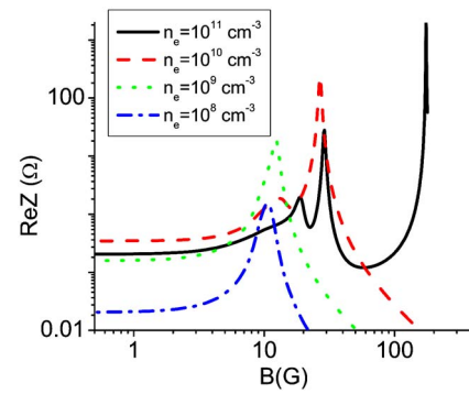
FIG. 4. (Color online). Surface resistance of warm bounded uniform Maxwellian plasmas for different electron densities as a function of the applied magnetic field. Discharge parameters: rf field frequency \omega/2\pi = 29 \text{ MHz} , electron temperature T_e = 4 \text{ eV} , electron collision frequency \nu = 1.2 \times 10^7 \text{ s}^{-1} , and the plasma half-length L/2 = 10.5 \text{ cm} .
