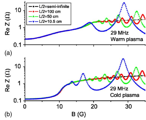
FIG. 2. (Color online). Surface resistance of semi-infinite and bounded plasmas of different lengths as a function of the applied magnetic field for a uniform plasma with a Maxwellian EEDF. The discharge frequency is 29 MHz, the plasma density n_e = 10^{11} cm ^{-3} , and the electron collision frequency \nu = 1.2 \times 10^7 s ^{-1} . (a) Warm plasma with the electron temperature T_e = 4 eV and (b) cold plasma with the electron temperature T_e \rightarrow 0 (local approximation for electron current).
