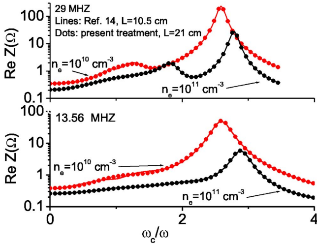
FIG. 1. (Color online). Surface resistance as a function of a normalized electron-cyclotron frequency. The solid lines correspond to the formalism of Ref. 14 for one grounded electrode with plasma length L/2 and the dotted lines correspond to the case of two driven electrodes with plasma length L . Shown: rf driving frequencies 29 and 13.56 MHz, electron temperature T_e = 4 eV, and electron collision frequency \nu = 1.2 \times 10^7 s ^{-1} .
