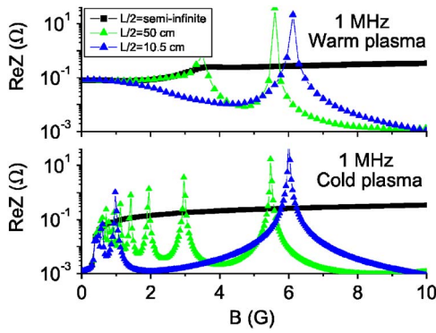
FIG. 3. (Color online). Surface resistance of semi-infinite and bounded plasmas of different lengths as a function of the applied magnetic field for a uniform plasma with a Maxwellian EEDF. The discharge frequency is 1 MHz, the plasma density n_e = 10^{11} \text{ cm}^{-3} , and the electron collision frequency \nu = 1.2 \times 10^5 \text{ s}^{-1} . (a) Warm plasma with the electron temperature T_e = 4 \text{ eV} and (b) cold plasma with the electron temperature of T_e \rightarrow 0 (local approximation for electron current).
